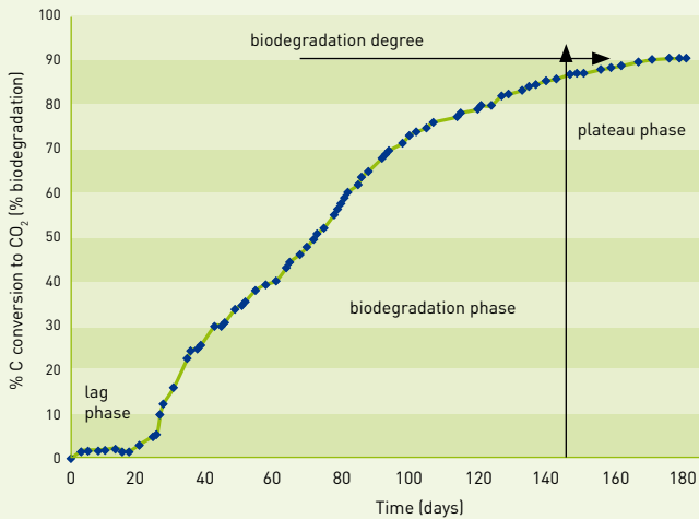
Figure 2: Test method to measure the rate and extent of microbial utilization (biodegradation) of biodegradable plastics
